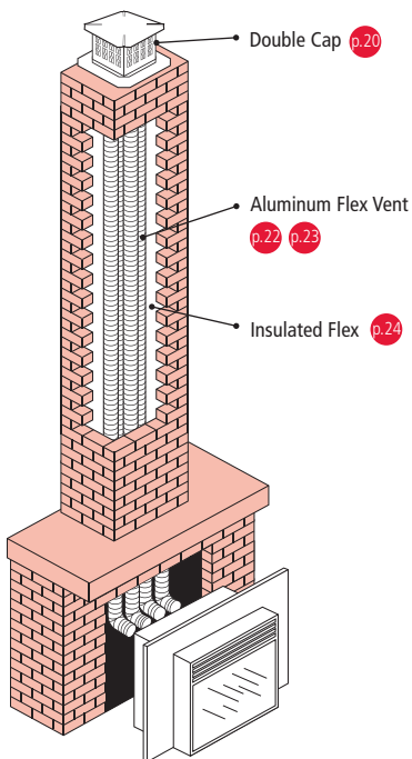
Back-to-back Application with Double Cap
